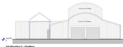
GA Elevation C - Distillery 1:100
