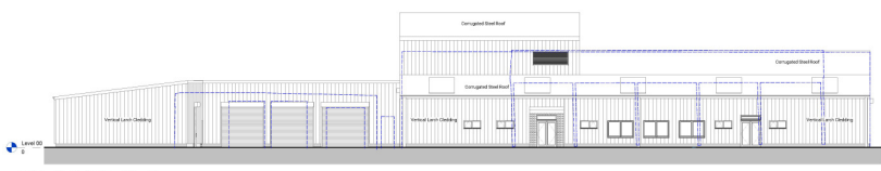
GA Elevation B - Distillery/Store 2 1:100
