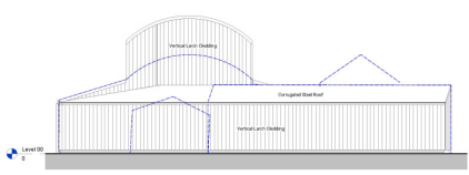
GA Elevation E - Store 2 1:100
